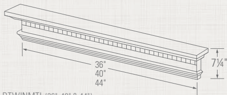
DTWINMTL (36", 40" & 44") Window Mantel with Dentil Strip
