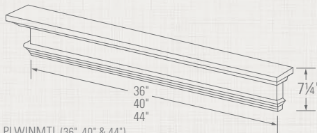
PLWINMTL (36", 40" & 44") Window Mantel
